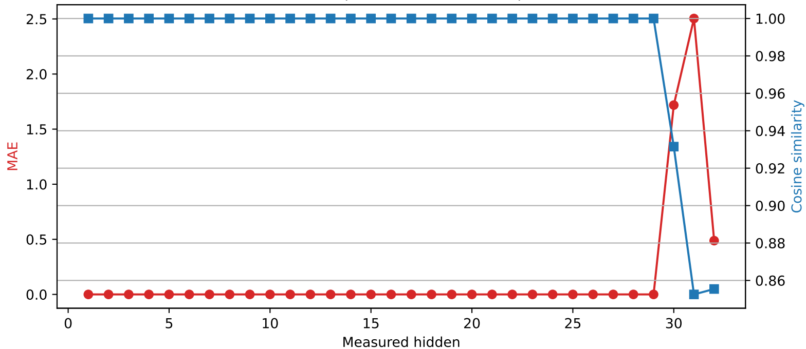
Phi-3-mini-4k-instruct | Quantized layer 29 | float64 → int4
