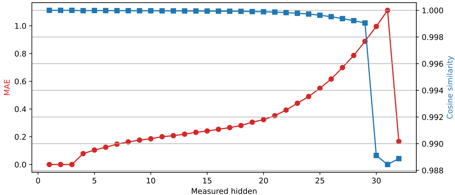
Phi-3-mini-4k-instruct | Quantized layer 3 | float64 → int4
