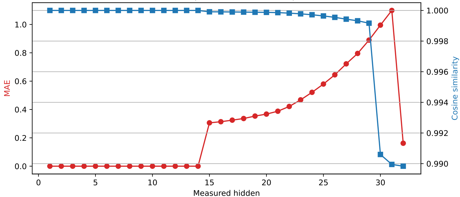
Phi-3-mini-4k-instruct | Quantized layer 14 | float64 \rightarrow int4
