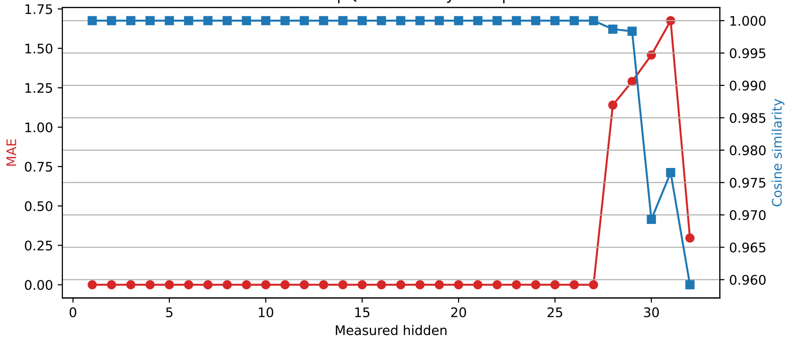
Phi-3-mini-4k-instruct | Quantized layer 27 | float64 \rightarrow int4
