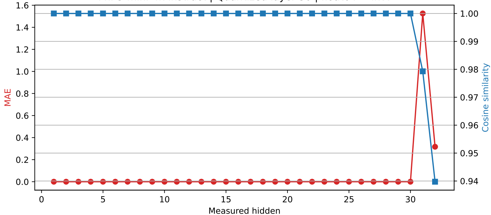
Phi-3-mini-4k-instruct | Quantized layer 30 | float64 → int4
