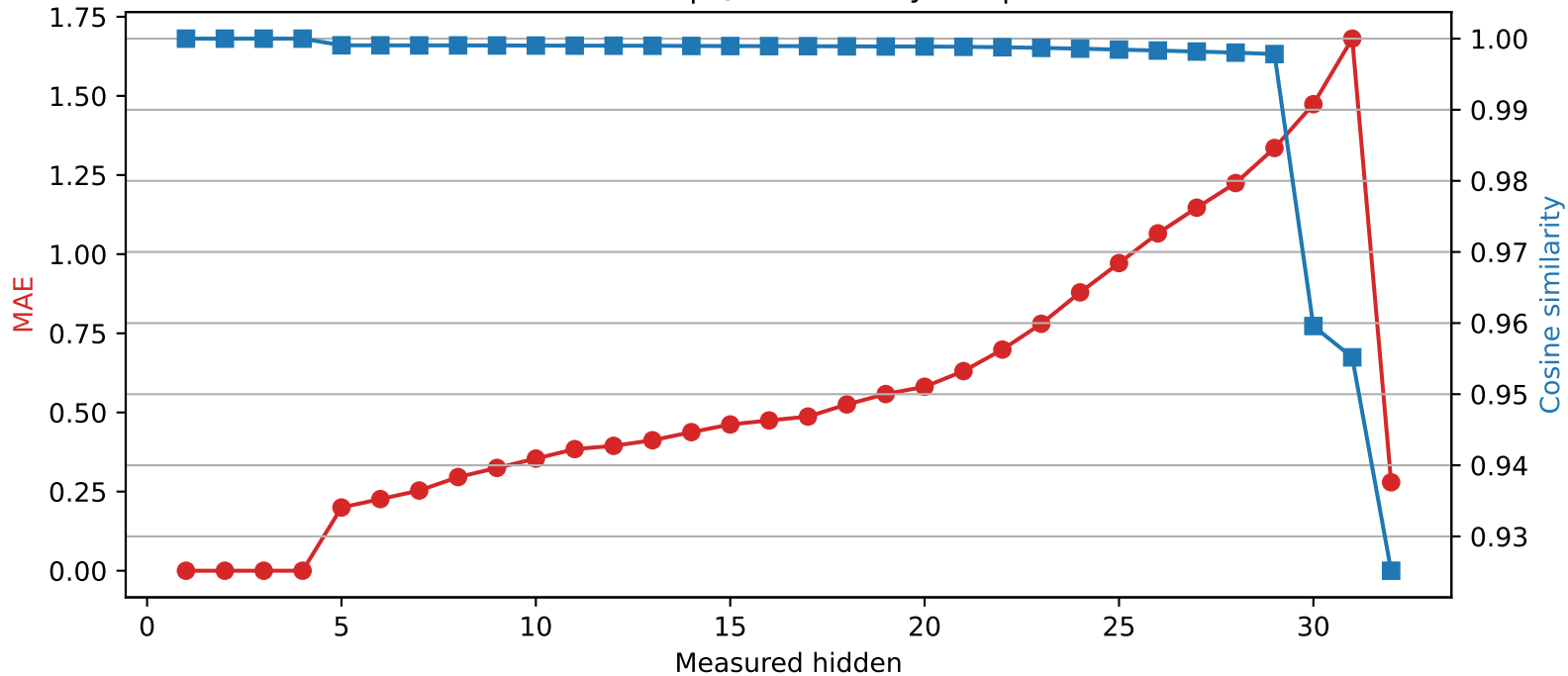
Phi-3-mini-4k-instruct | Quantized layer 4 | float64 → int4
