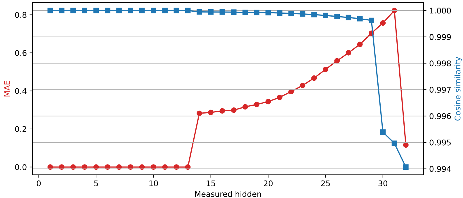
Phi-3-mini-4k-instruct | Quantized layer 13 | float64 → int4
