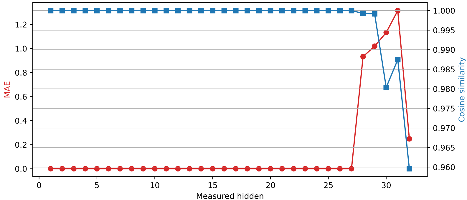
Phi-3-mini-4k-instruct | Quantized layer 27 | float64 → int4
