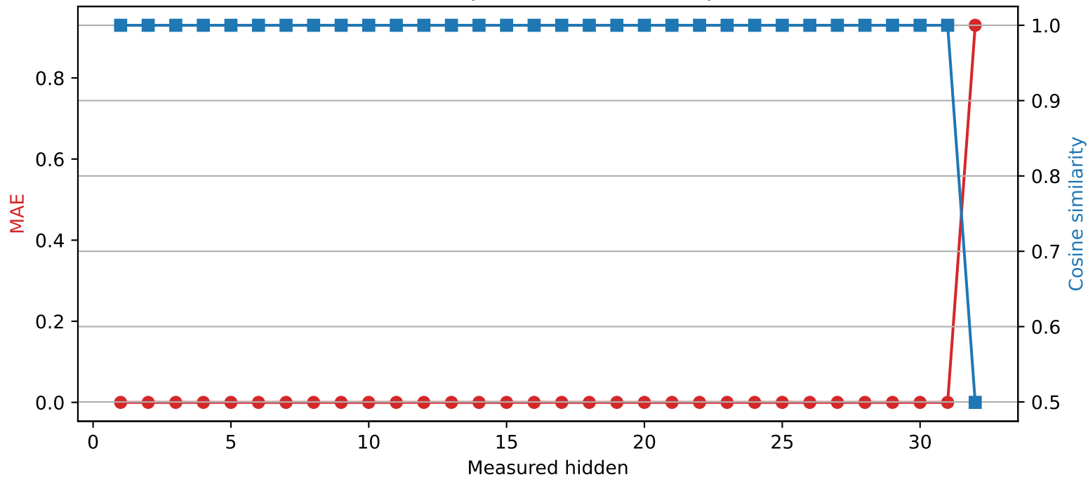
Phi-3-mini-4k-instruct | Quantized layer 31 | float64 \rightarrow int4
