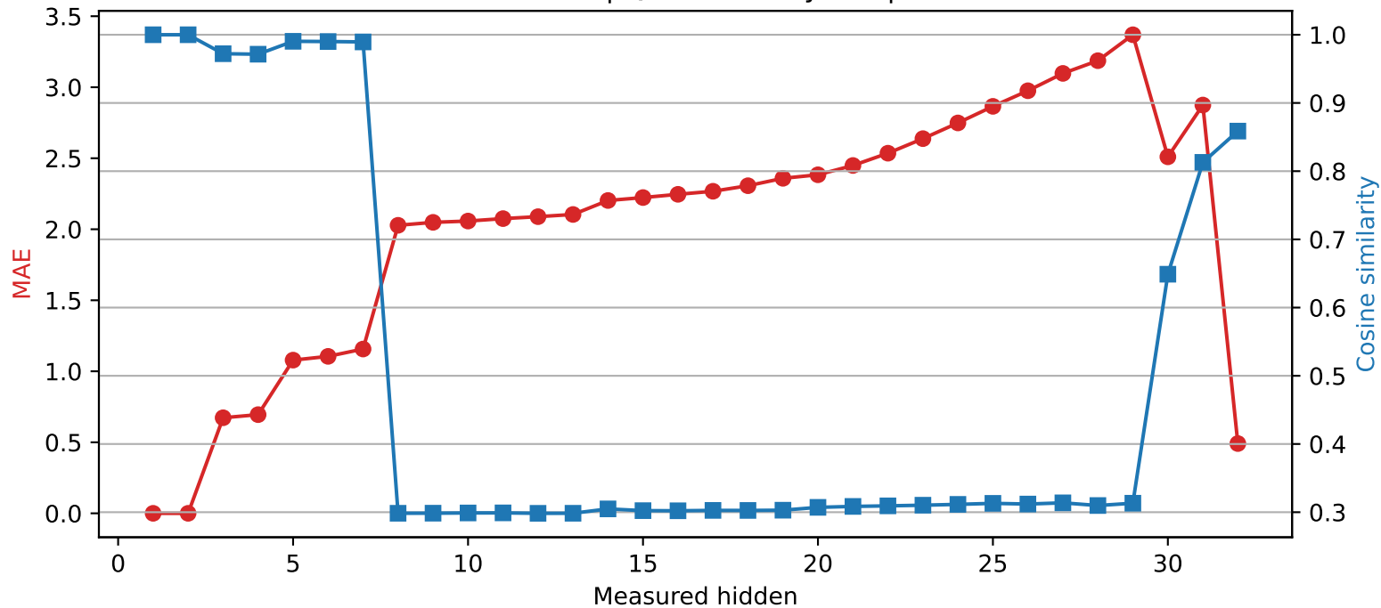
Phi-3-mini-4k-instruct | Quantized layer 2 | float16 \rightarrow int2
