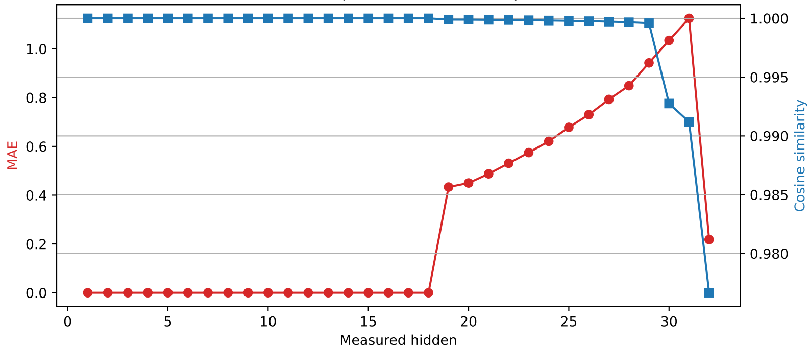
Phi-3-mini-4k-instruct | Quantized layer 18 | float16 \rightarrow int2
