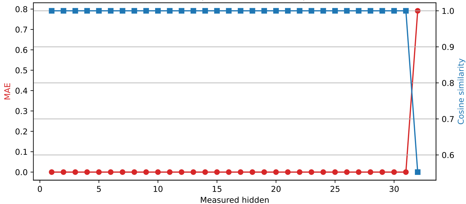
Phi-3-mini-4k-instruct | Quantized layer 31 | float16 \rightarrow int2
