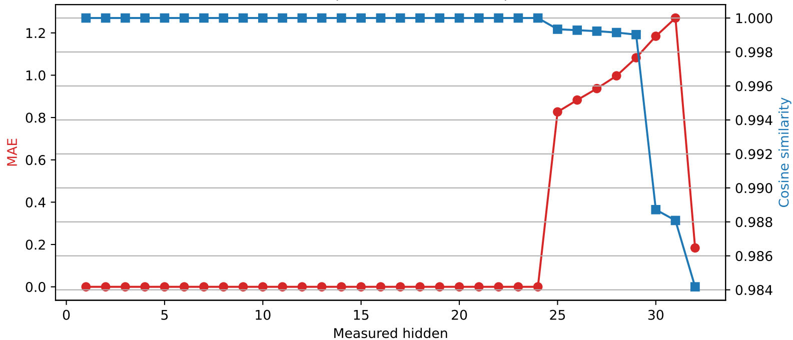
Phi-3-mini-4k-instruct | Quantized layer 24 | float16 → int2
