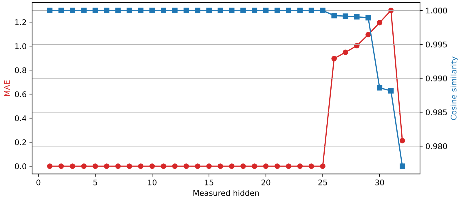
Phi-3-mini-4k-instruct | Quantized layer 25 | float16 → int2
