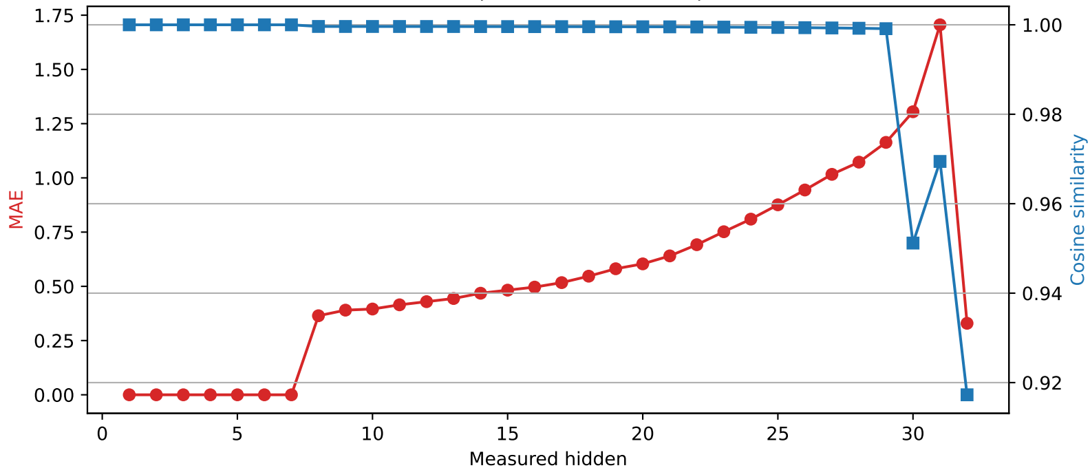
Phi-3-mini-4k-instruct | Quantized layer 7 | float32 \rightarrow int2
