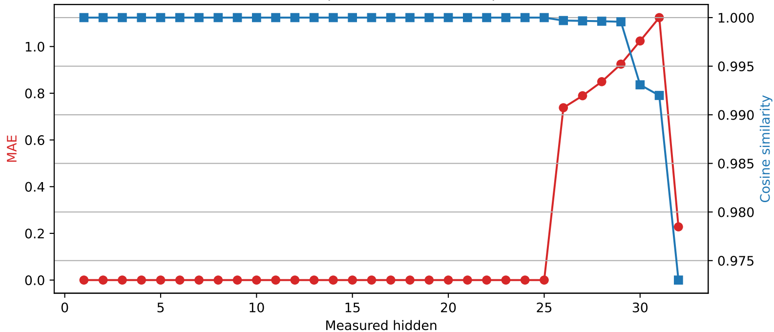
Phi-3-mini-4k-instruct | Quantized layer 25 | float32 → int2
