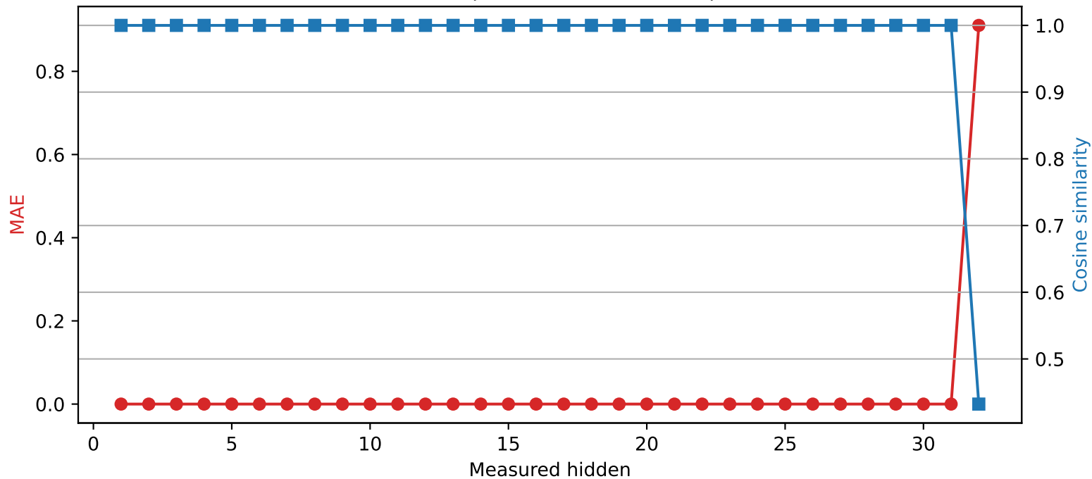
Phi-3-mini-4k-instruct | Quantized layer 31 | float32 \rightarrow int2
