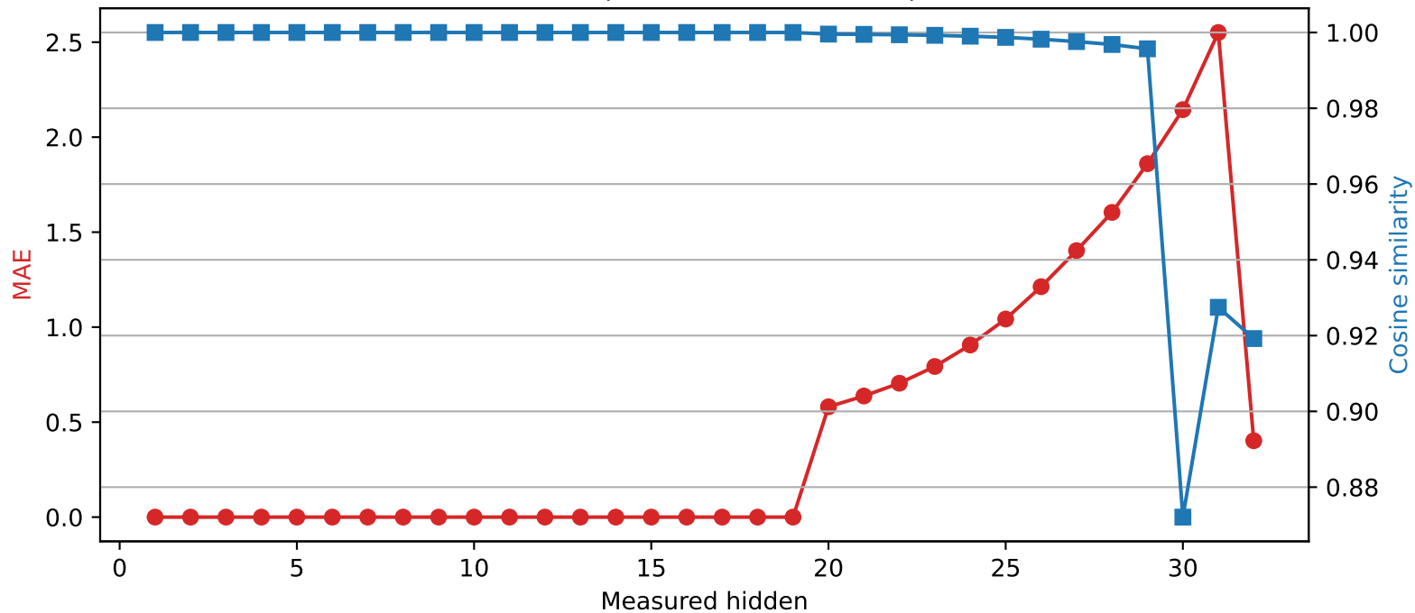
Phi-3-mini-4k-instruct | Quantized layer 19 | float32 → int2
