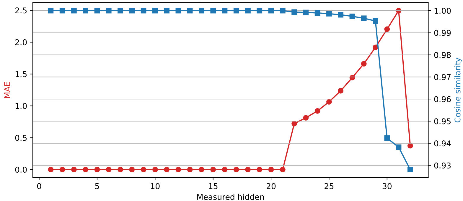
Phi-3-mini-4k-instruct | Quantized layer 21 | float32 \rightarrow int2
