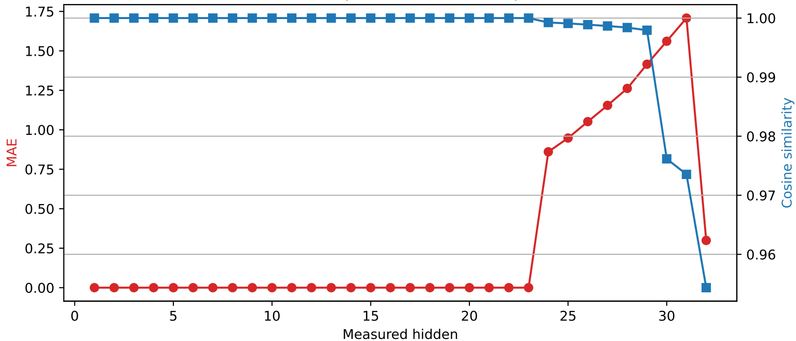
Phi-3-mini-4k-instruct | Quantized layer 23 | float32 \rightarrow int2
