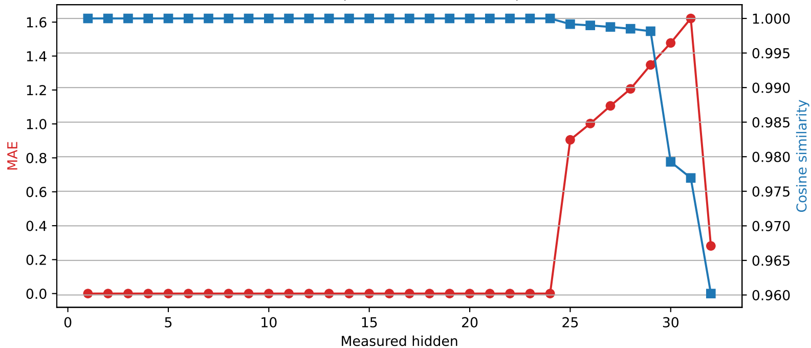
Phi-3-mini-4k-instruct | Quantized layer 24 | float32 \rightarrow int2
