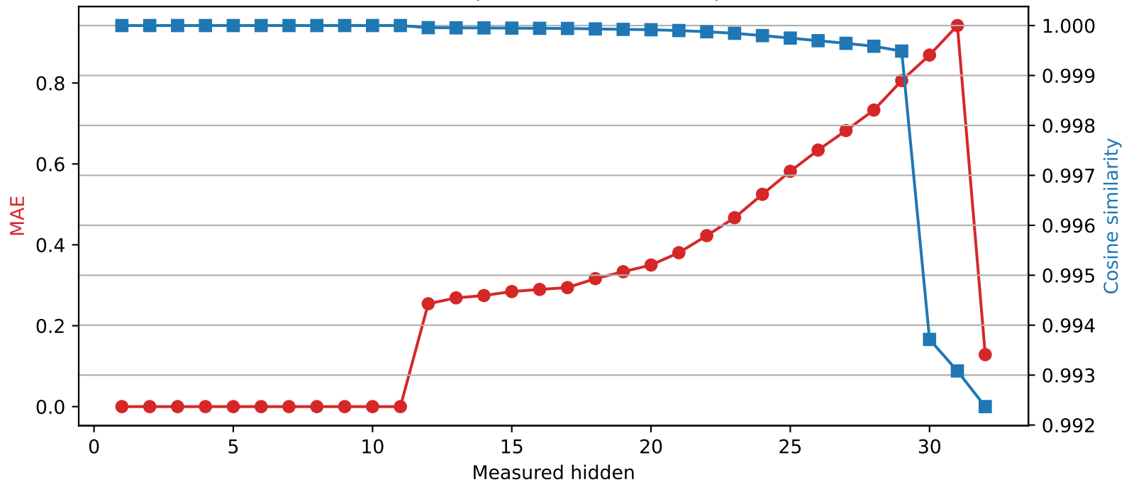
Phi-3-mini-4k-instruct | Quantized layer 11 | float32 → int2
