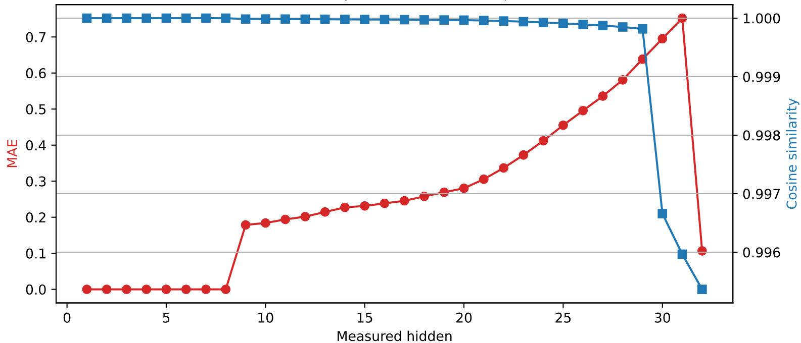
Phi-3-mini-4k-instruct | Quantized layer 8 | float64 \rightarrow int2
