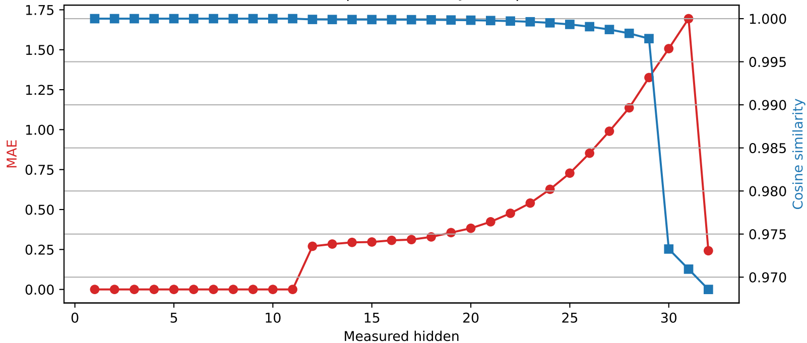
Phi-3-mini-4k-instruct | Quantized layer 11 | float64 → int2
