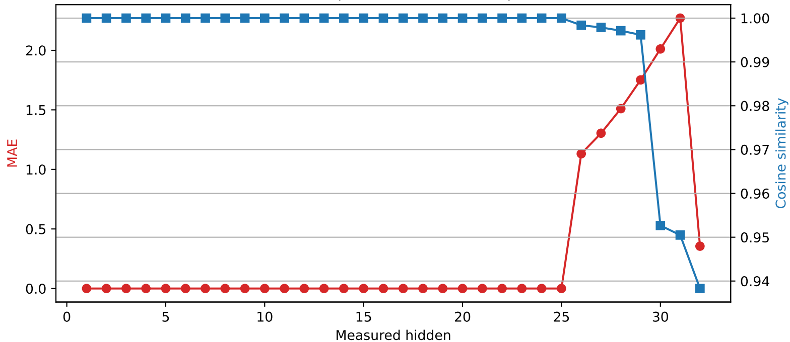
Phi-3-mini-4k-instruct | Quantized layer 25 | float64 → int2
