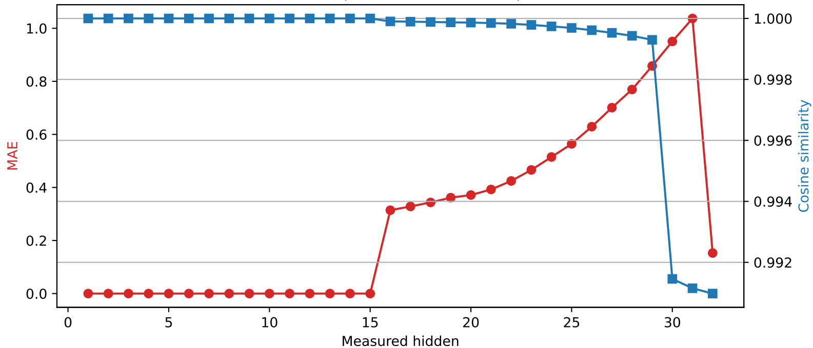
Phi-3-mini-4k-instruct | Quantized layer 15 | float64 \rightarrow int2
