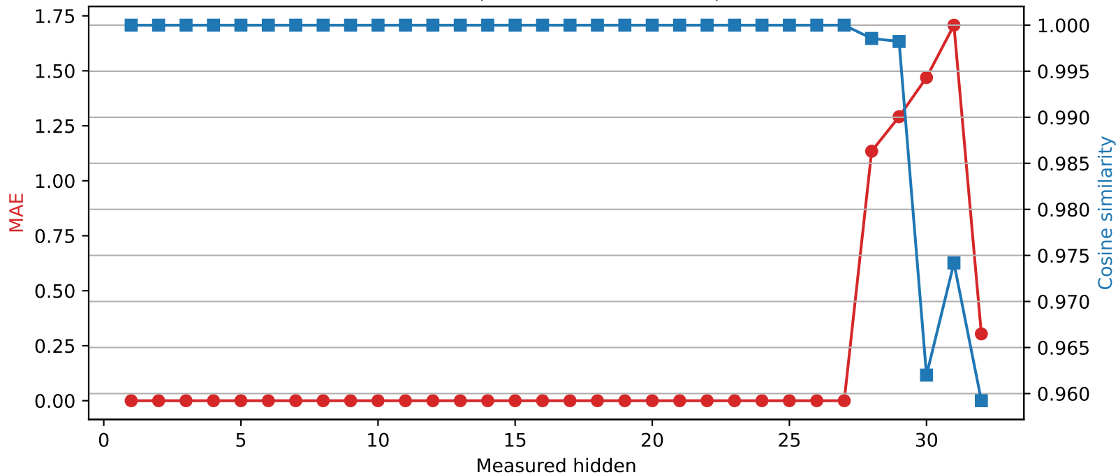
Phi-3-mini-4k-instruct | Quantized layer 27 | float64 → int2
