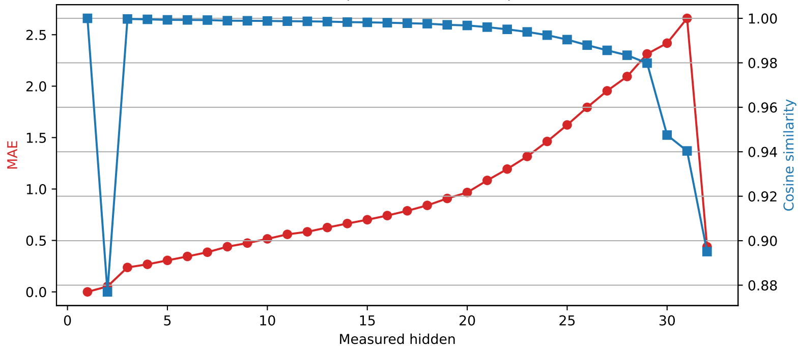
Phi-3-mini-4k-instruct | Quantized layer 1 | float64 → int2
