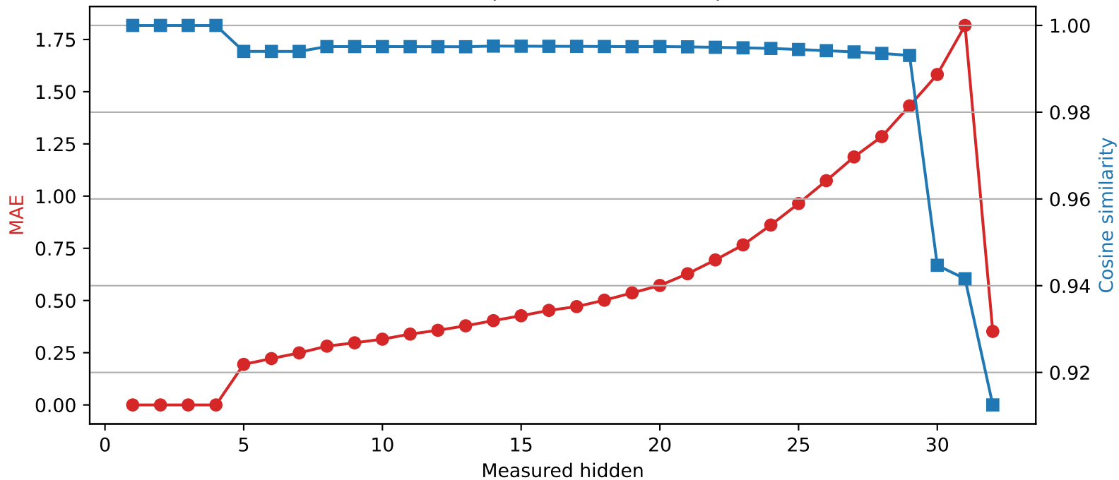
Phi-3-mini-4k-instruct | Quantized layer 4 | float64 → int2
