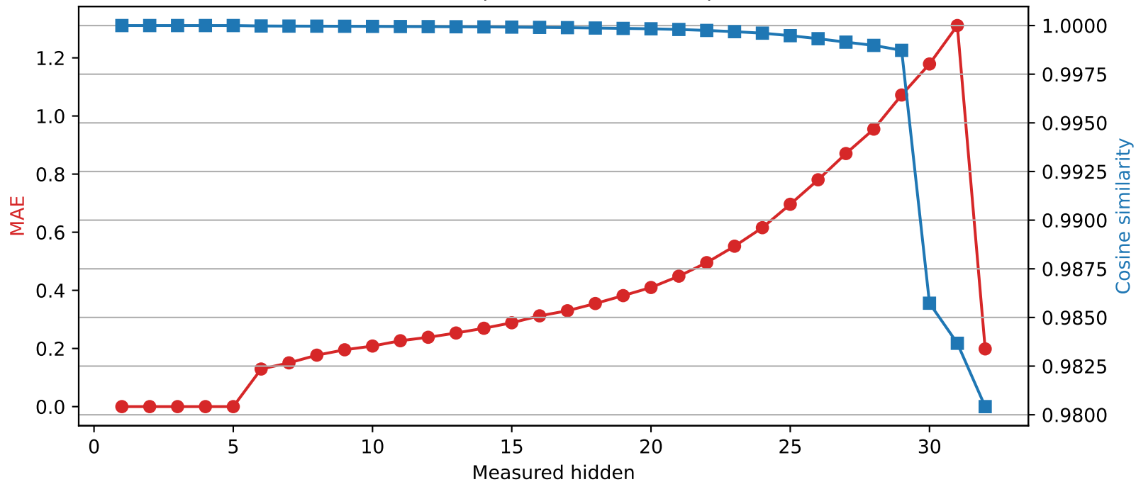
Phi-3-mini-4k-instruct | Quantized layer 5 | float64 → int2
