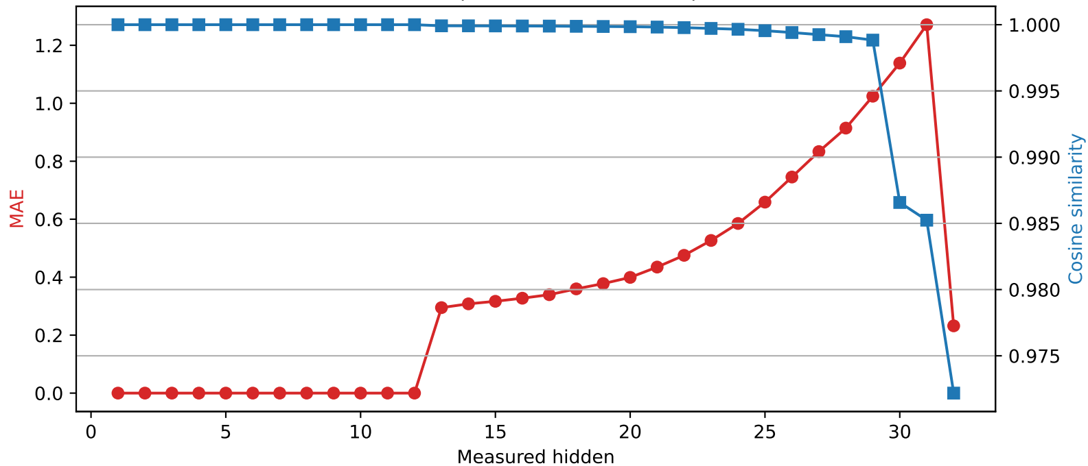
Phi-3-mini-4k-instruct | Quantized layer 12 | float64 → int2
