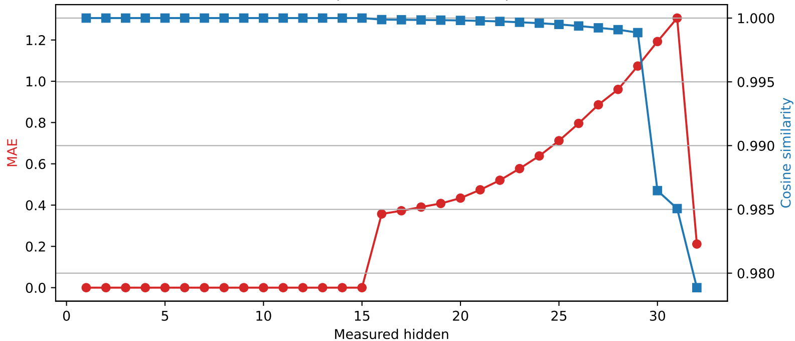
Phi-3-mini-4k-instruct | Quantized layer 15 | float64 → int2
