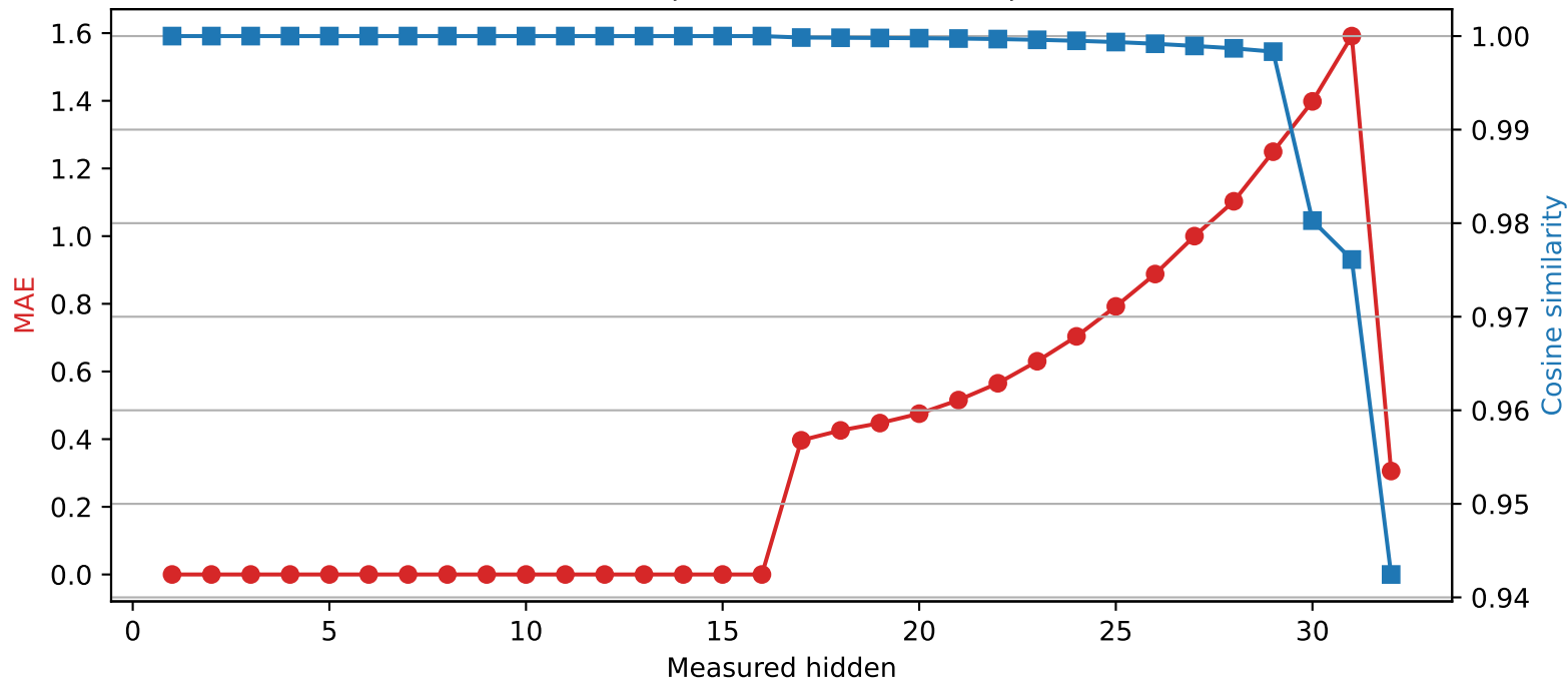
Phi-3-mini-4k-instruct | Quantized layer 16 | float64 → int2
