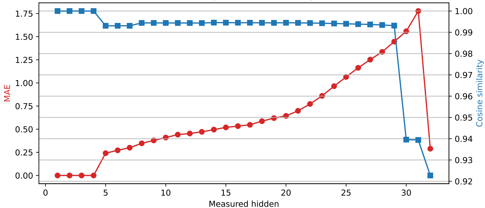
Phi-3-mini-4k-instruct | Quantized layer 4 | float64 \rightarrow int2
