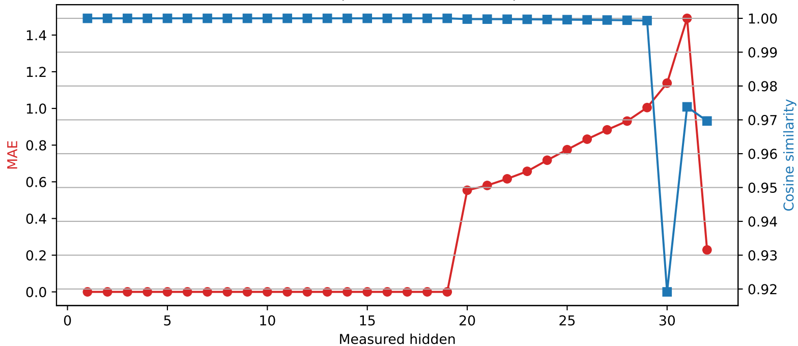
Phi-3-mini-4k-instruct | Quantized layer 19 | float64 → int2
