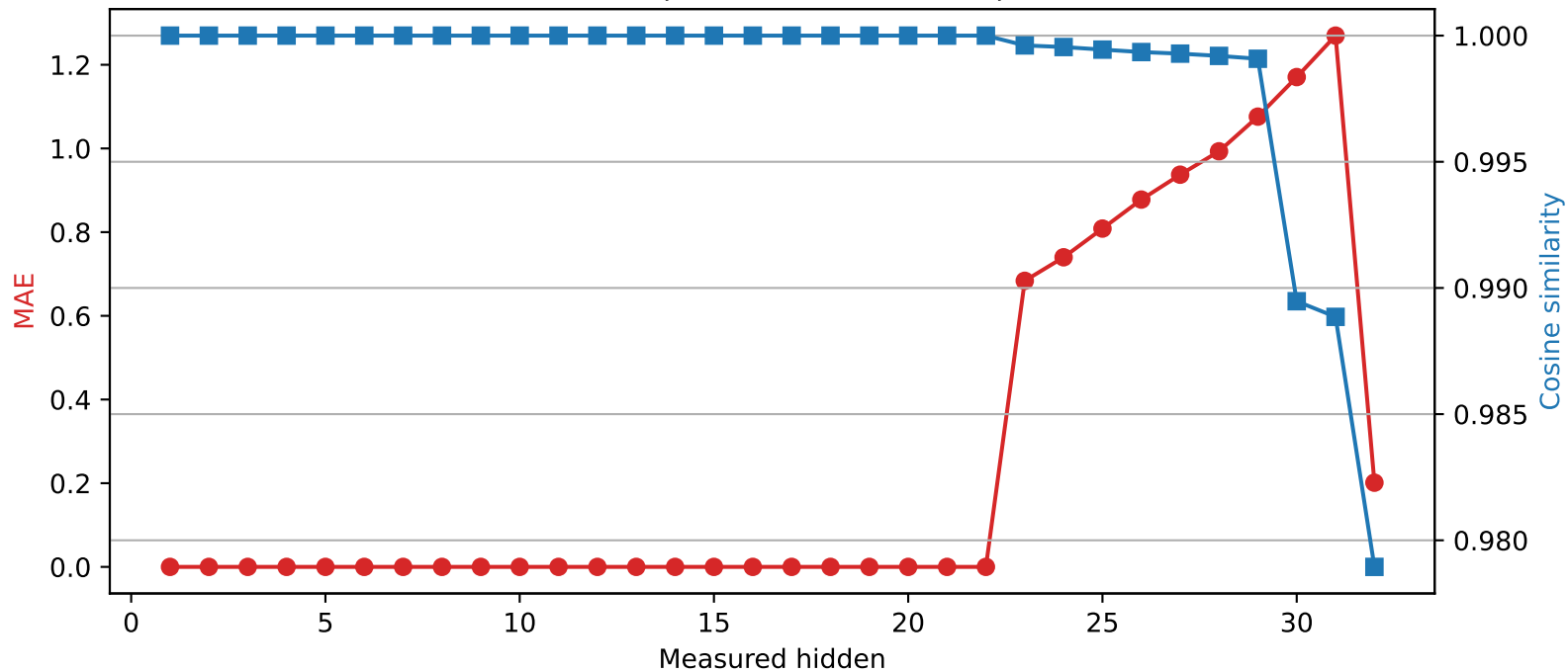
Phi-3-mini-4k-instruct | Quantized layer 22 | float64 → int2
