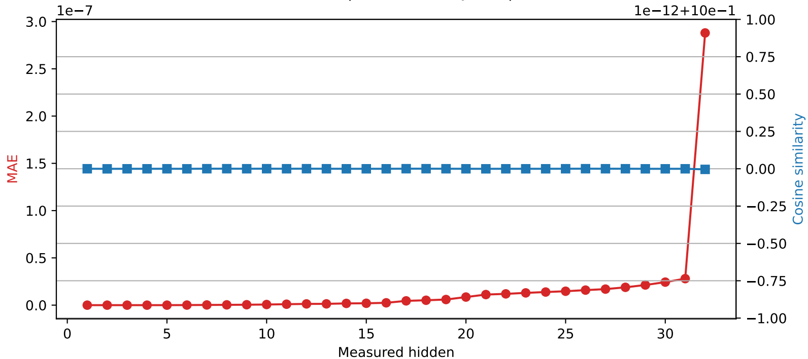
Mistral-7B-Instruct-v0.3 | Quantized layer 5 | float64 → int32
