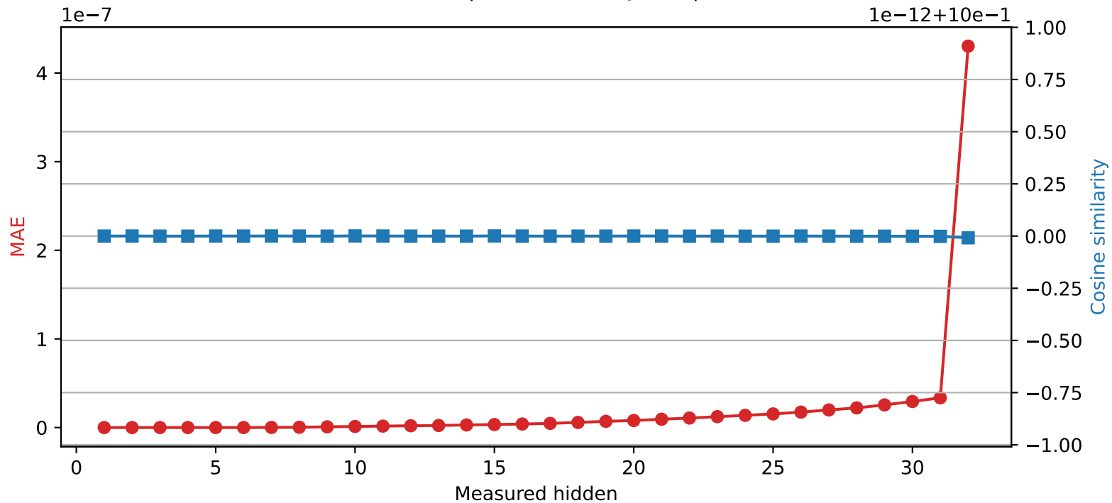
Mistral-7B-Instruct-v0.3 | Quantized layer 6 | float64 → int32
