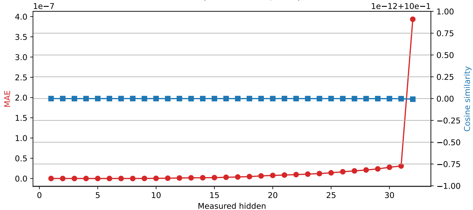
Mistral-7B-Instruct-v0.3 | Quantized layer 8 | float64 → int32
