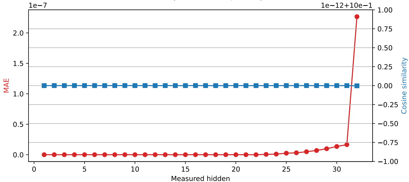
Mistral-7B-Instruct-v0.3 | Quantized layer 22 | float64 → int32
