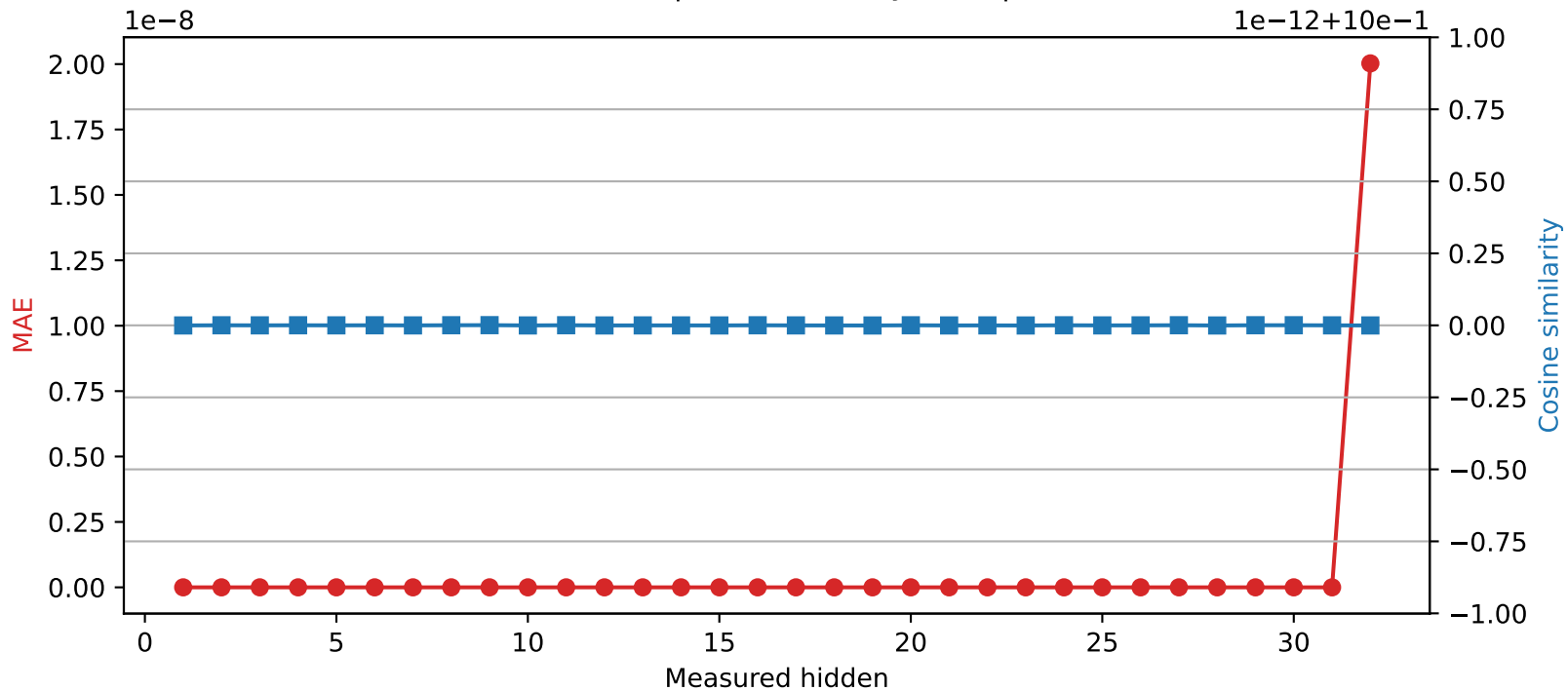
Mistral-7B-Instruct-v0.3 | Quantized layer 31 | float64 → int32
