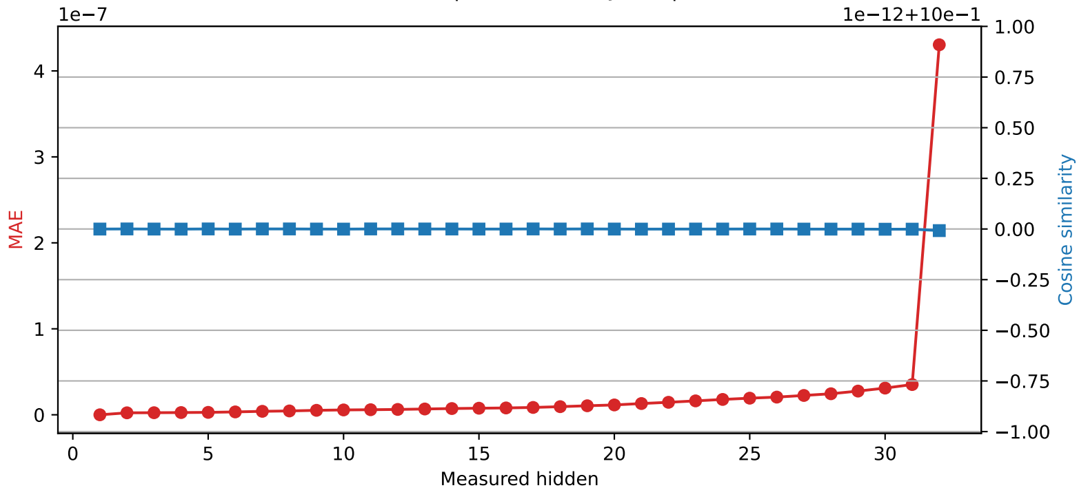
Mistral-7B-Instruct-v0.3 | Quantized layer 1 | float64 → int32
