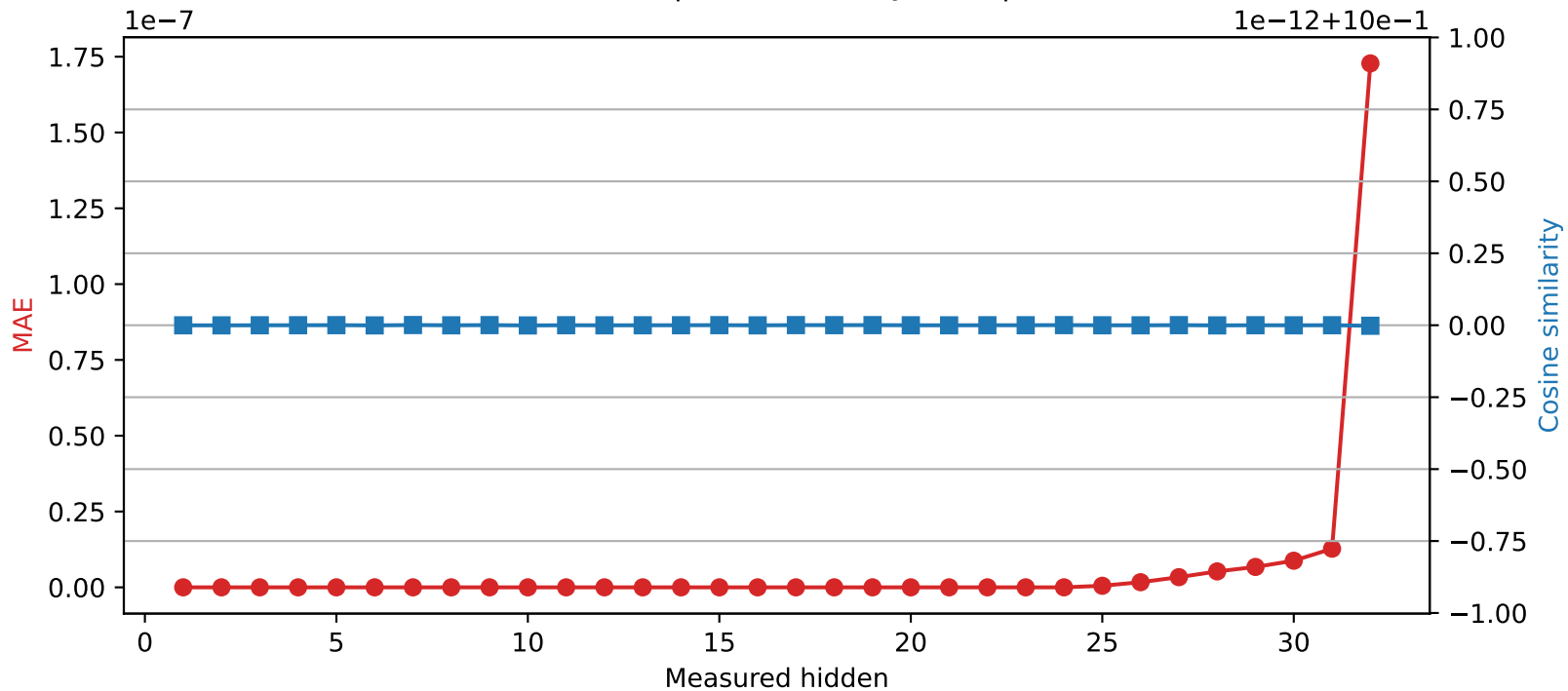
Mistral-7B-Instruct-v0.3 | Quantized layer 24 | float64 → int32
