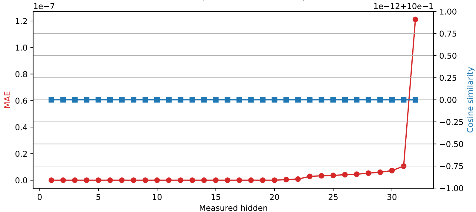
Mistral-7B-Instruct-v0.3 | Quantized layer 20 | float64 → int32
