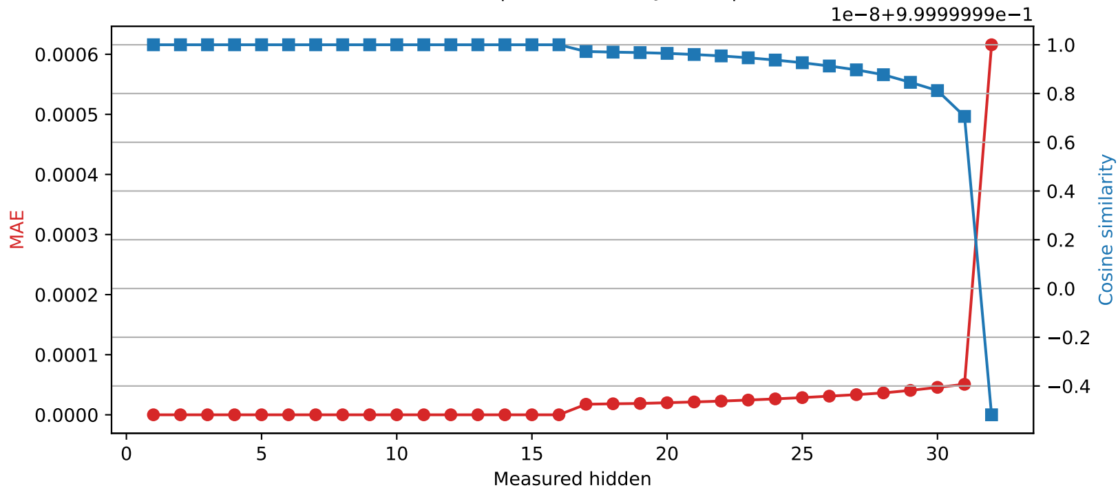
Mistral-7B-Instruct-v0.3 | Quantized layer 16 | float32 → int16
