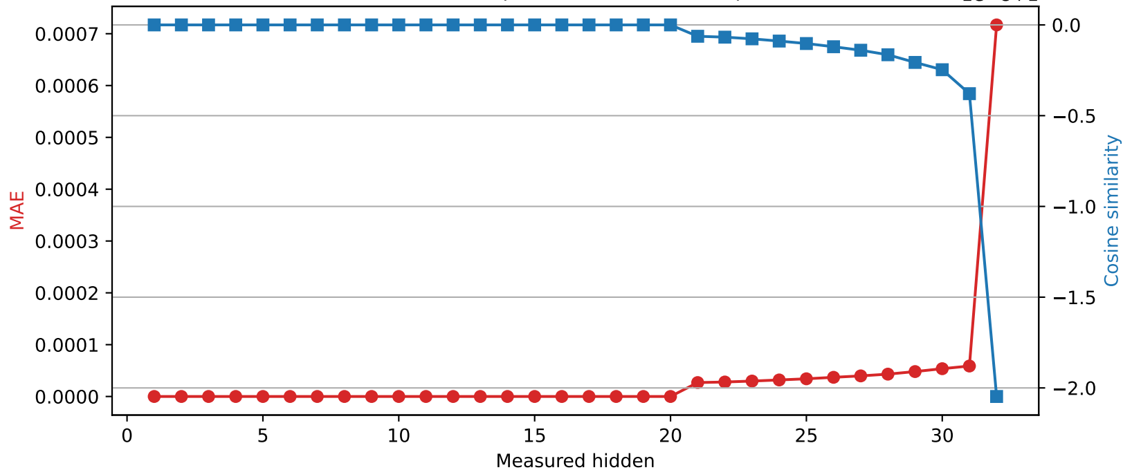
Mistral-7B-Instruct-v0.3 | Quantized layer 20 | float32 → int16
