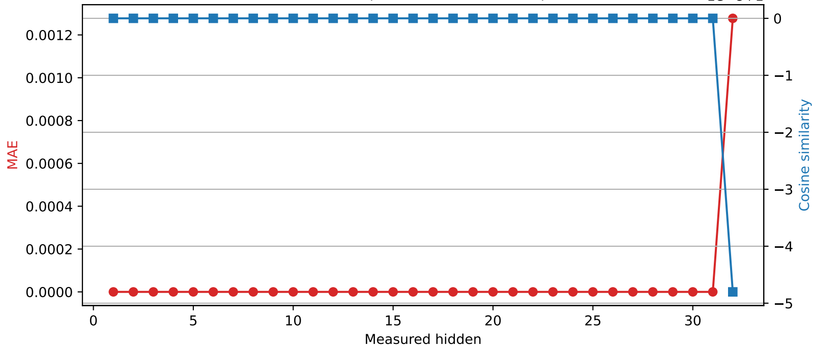
Mistral-7B-Instruct-v0.3 | Quantized layer 31 | float32 → int16
