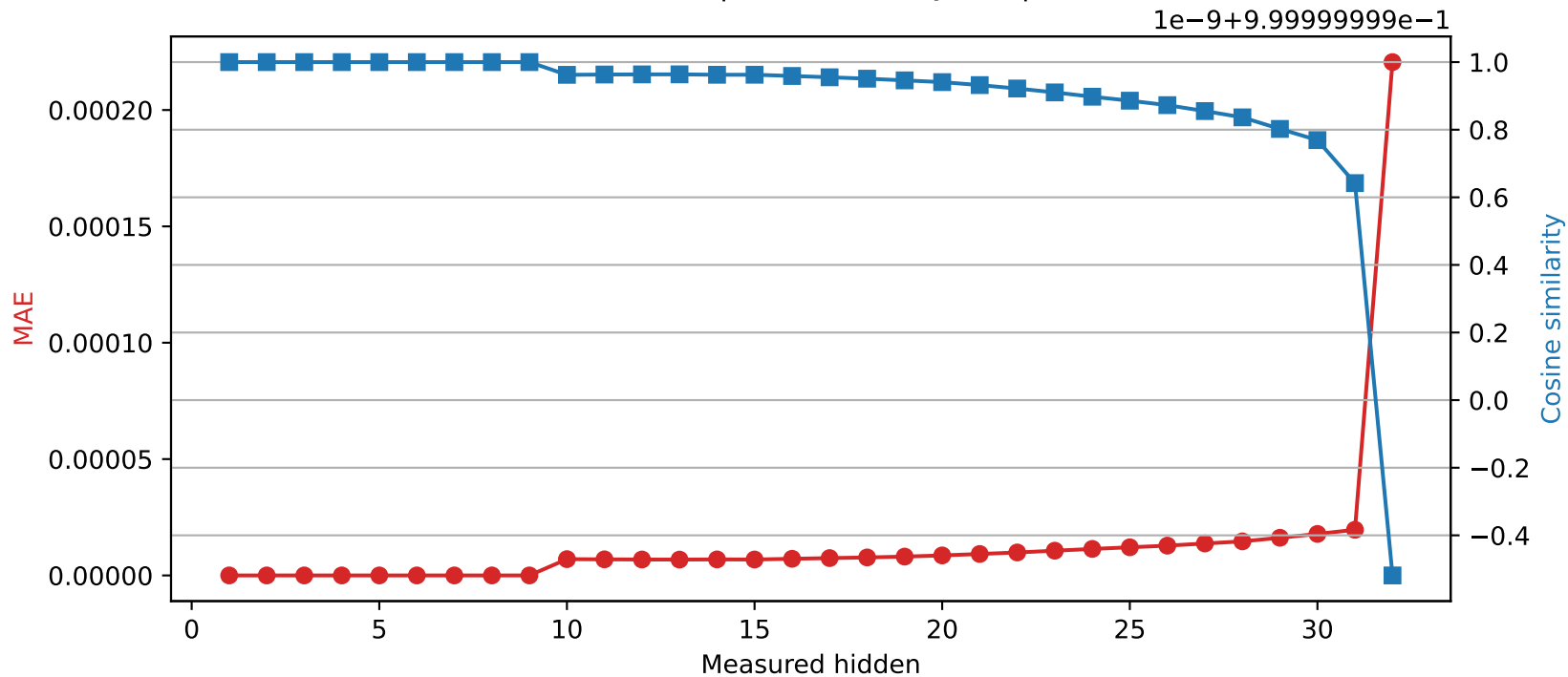
Mistral-7B-Instruct-v0.3 | Quantized layer 9 | float32 → int16
