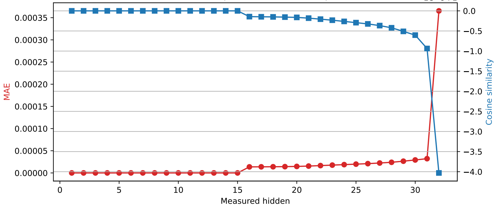
Mistral-7B-Instruct-v0.3 | Quantized layer 15 | float32 → int16
