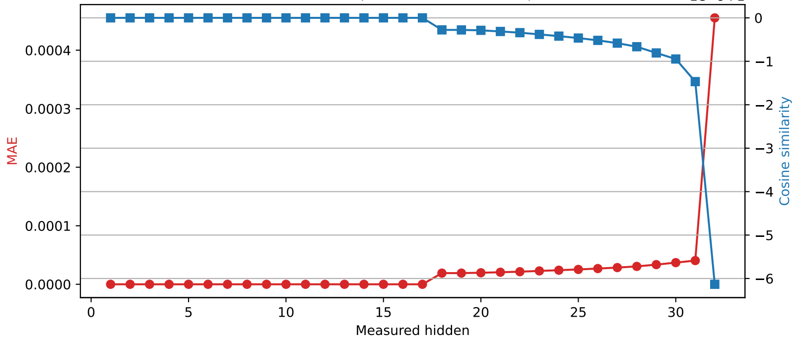
Mistral-7B-Instruct-v0.3 | Quantized layer 17 | float32 → int16
